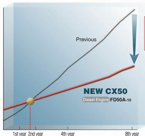
Komatsu tested data, Comparison with FD50A-8 model. Operation hours: 5 h/day, 25 days/month (Total: Approx. 1500 h/year). Maintenance intervals to manufacturer's recommendation. Cost calculation is based on Japanese market price. The results may vary depending on conditions.
